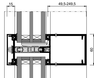
transom – cross-section
