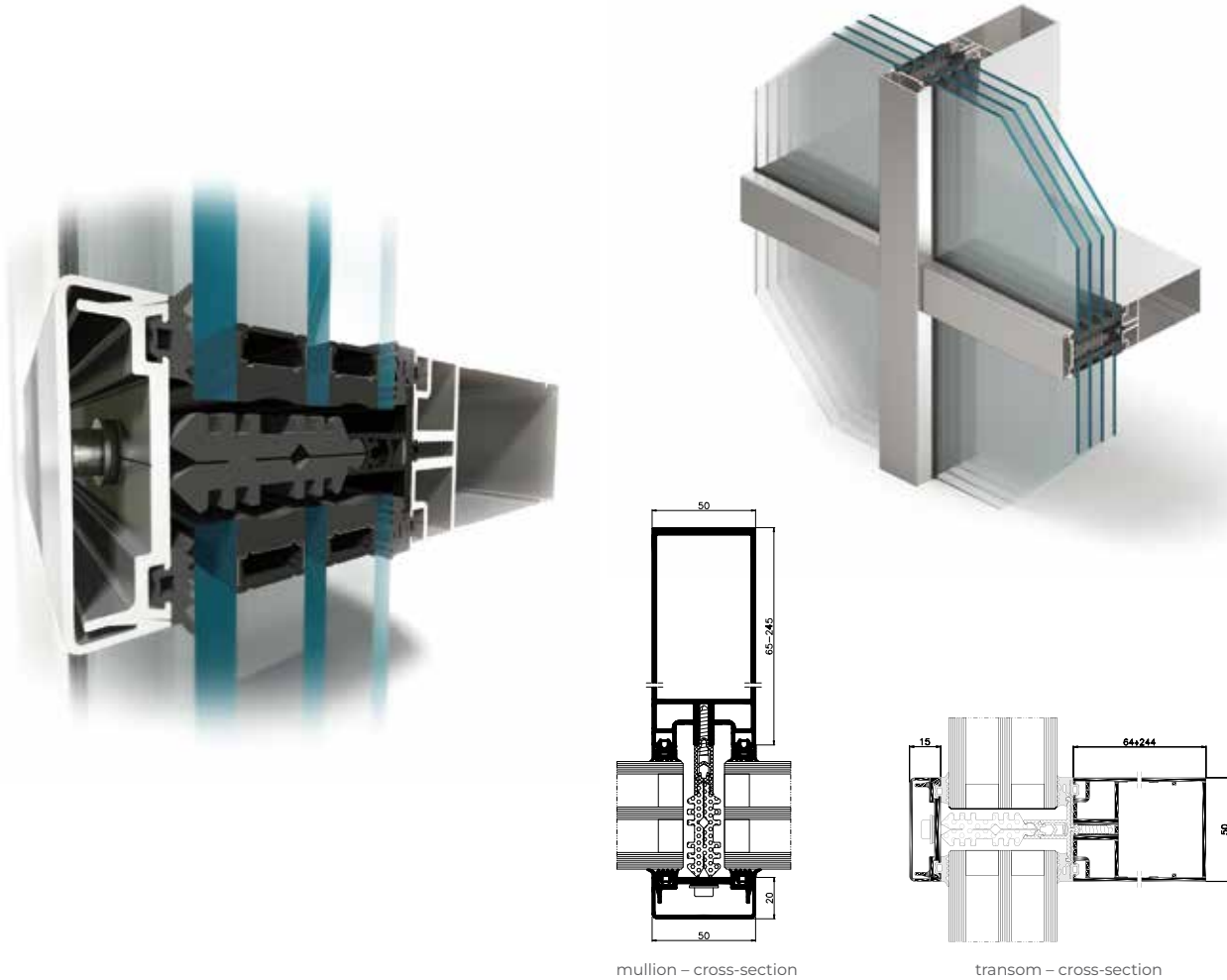
mullion – cross-section
