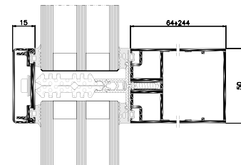
transom – cross-section
