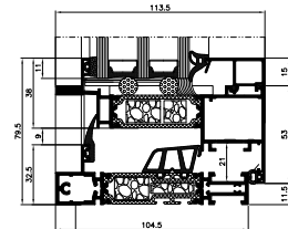
opening window - cross section
