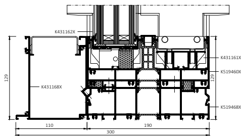
cross section of the bottom of the door
