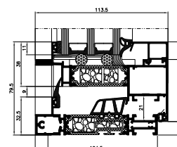
opening window - cross section
