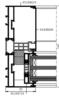
cross section of the side of the door
